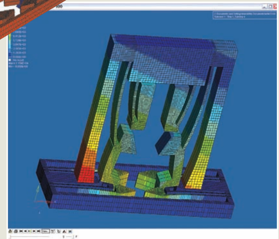
Zyxex engineers develop finite-element models with Altair HyperMesh (left) and visualize results with Altair HyperView (below).
